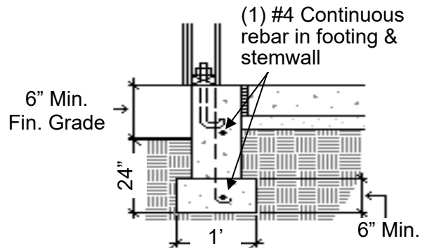
STEMWALL FOOTING UNHEATED
