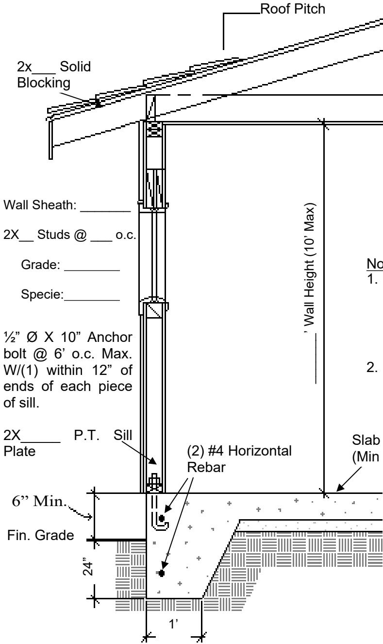
WALL SECTION – MONOLITHIC SLAB UNHEATED
